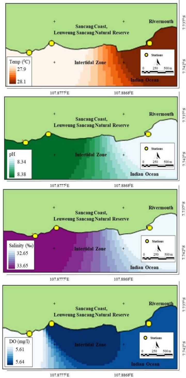
Figure 5. Spatial estimations of environmental variables include water temperature, pH, salinity, and DO at intertidal zones of Sancang Coast, Leuweung Sancang Natural Reserve, West Java, Indonesia.
