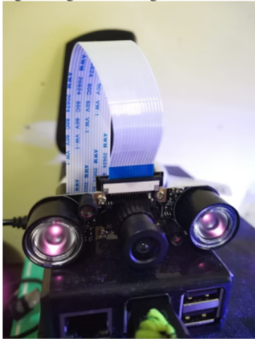
Fig. 3 Raspberry with a camera module equipped with an IR sensor
