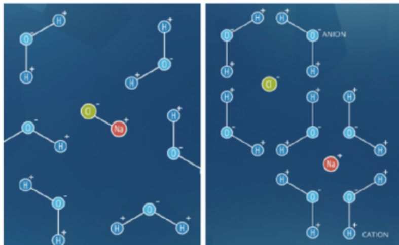
Fig. 1. Anions and cations formed in salt water [4].
