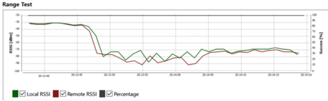
Fig. 11. The range result of the 3rd test using XCTU applications at a depth of 0-5 m.
