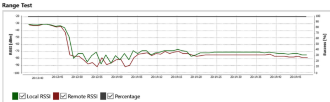
Fig. 10. The range result of the 2nd test using XCTU application at a depth of 0–5 m.
