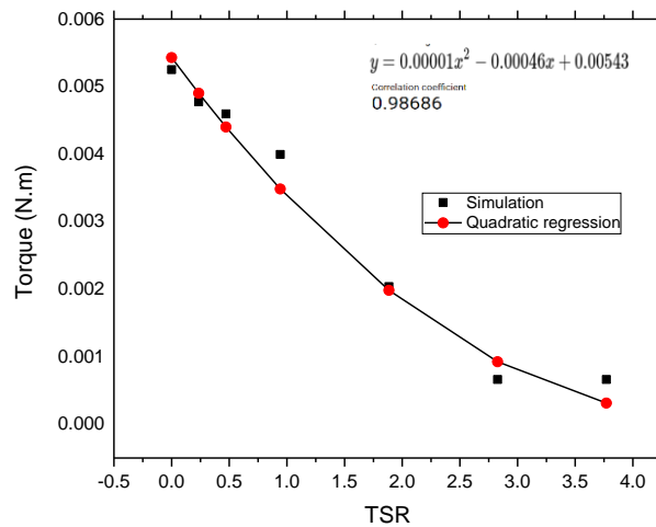
Fig. 11 Rotor torque vs. wind velocity
