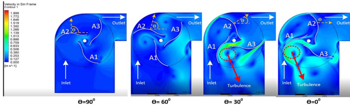
Fig. 13 Airspeeds on turbine blades under compressed conditions
