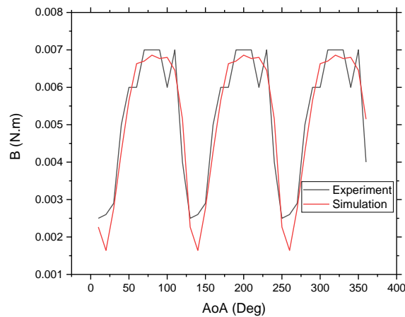
Fig. 9 Rotor torque vs. AoA
