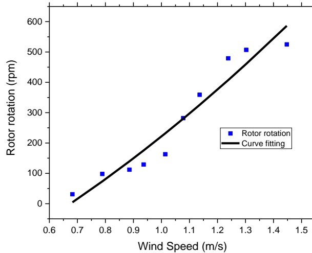
Fig. 12 Rotor rotation vs. airspeeds
