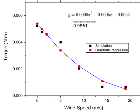
Fig. 10 Turbine torque vs. airspeeds
