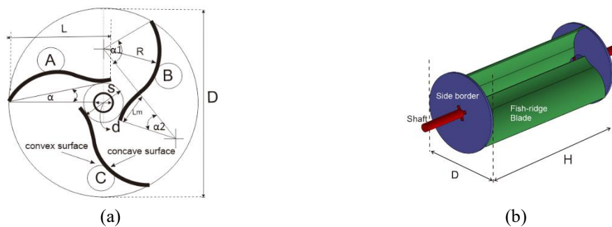
Fig. 4 The design of the fish-ridge turbine. (a). The side view of the fish-ridge turbine with overlap ratio (OR) and (b). Fish-ridge turbine 3D design
