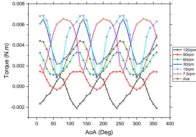
Fig. 7 Static torque vs. AoA at various rpm
