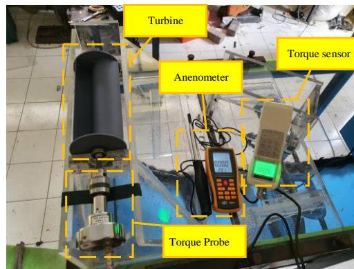
Fig. 8 The turbine static torque measurement on the OWC prototype
