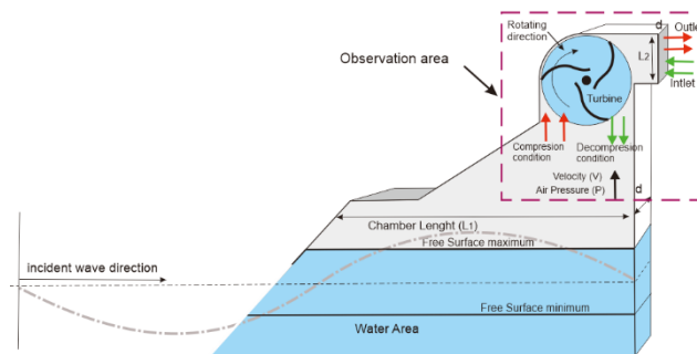
Fig. 2 The mechanism of the OWC with a fish-ridge turbine
