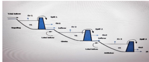
Fig. 4. A balance model of a multi-reservoir system.
