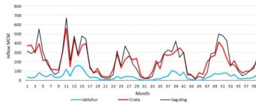
Fig. 6. Real inflow 2001 – 2005.
