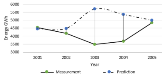
Fig. 7. Real energy and energy prediction in GWh.
