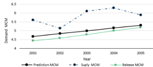
Fig. 8 Demand in year in Jatiluhur reservoir.
