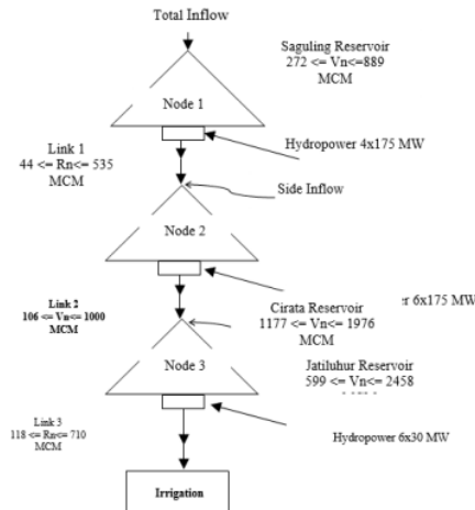
Fig. 3. Reservoir model
