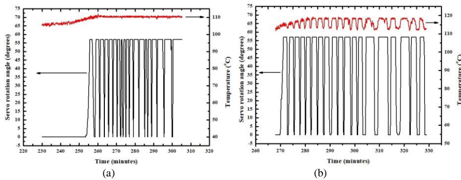
Figure 4. Open and close cycles of gas valve by servo rotation and changes in temperature around the set-point temperature of (a) 110°C.
