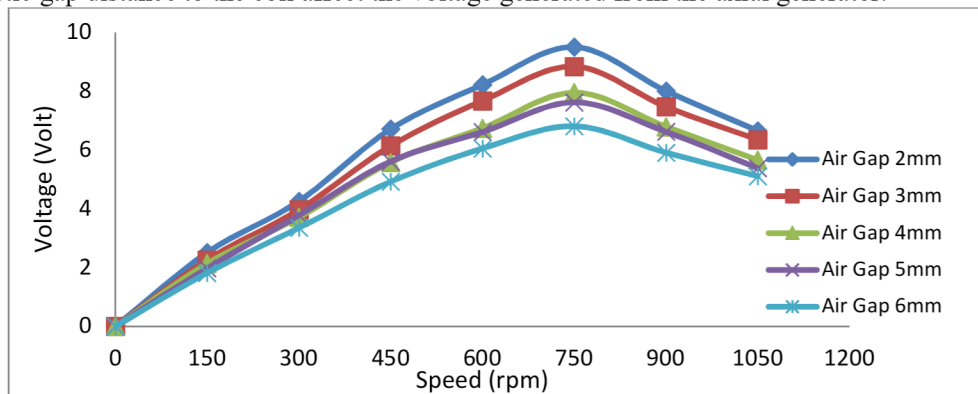
Figure 9. Relationship between output voltage and speed (rpm).
