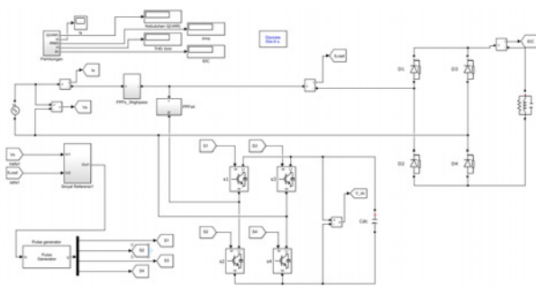
Fig. 4. Model implementation in SIMULINK
