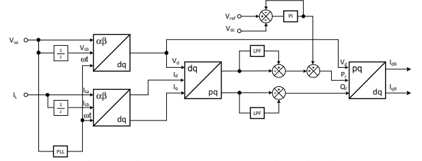
Fig 2. Reference Current Generation Circuit
