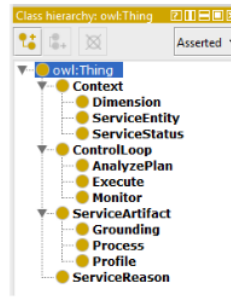
Figure 2: Class hierarchy of self-adaptive service knowledge.
