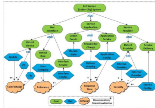
Figure 5: Modeling IoT services based on the goal model.
