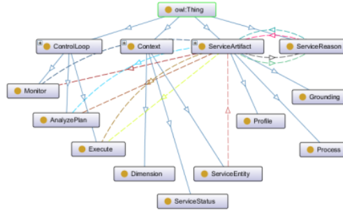
Figure 3: OntoGraf of self-adaptive service knowledge.
