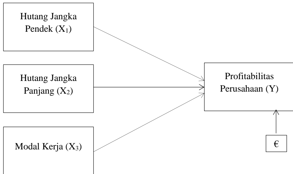
Gambar 3.1 Paradigma Penelitian
