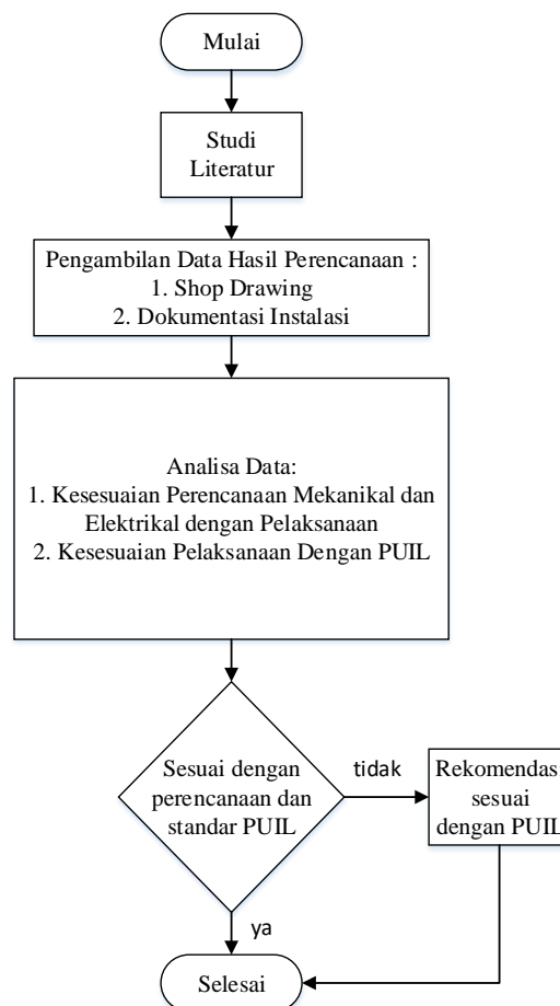
Gambar 3. 1 Fowchart Penelitian
