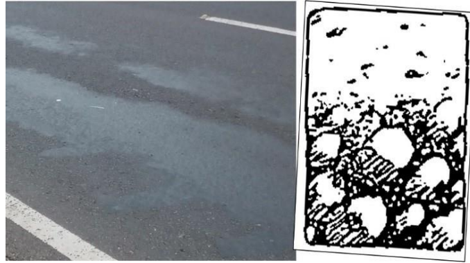
Gambar 2.27 Pengausan ( Polished Agregat )
