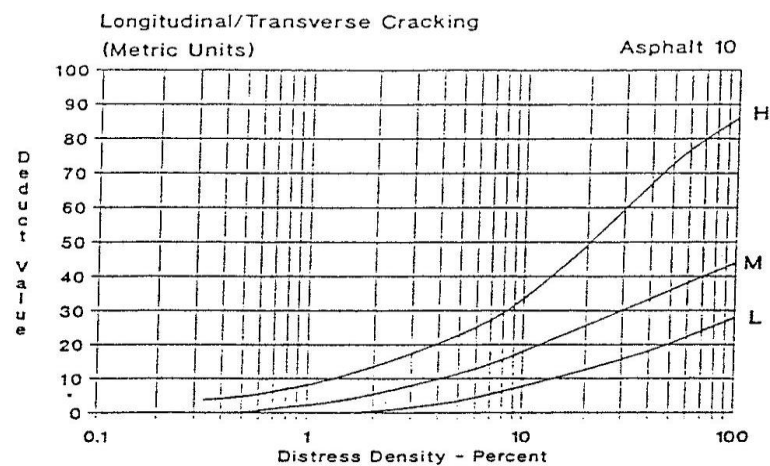
Gambar 2.24 Deduct Value Longitudinal and Transverse Cracking
