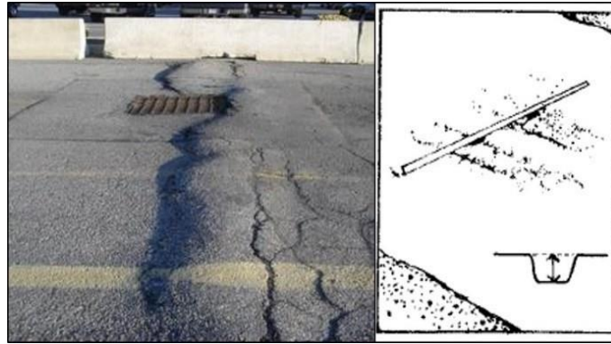
Gambar 2.32 Alur ( Rutting )
