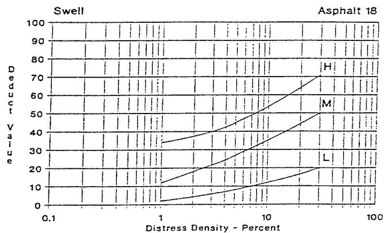
Gambar 2.38 Deduct Value Swell
