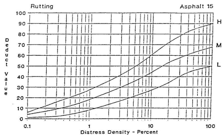
Gambar 2.33 Deduct Value Rutting
