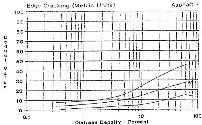
Gambar 2.21 Deduct Value Retak Pinggir Edge Cracking
