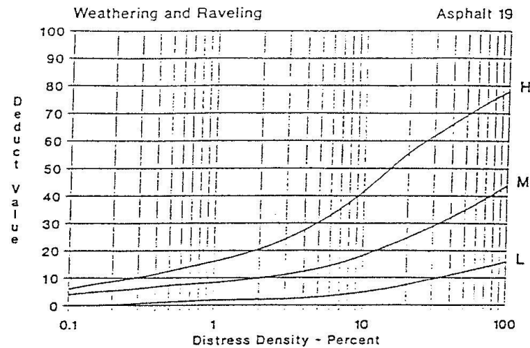
Gambar 2.40 Deduct Value Raveling and Weathering
