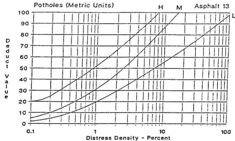
Gambar 2.30 Deduct Value Potholes
