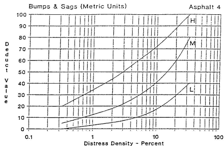
Gambar 2.15 Deduct Value Bump and Sags
