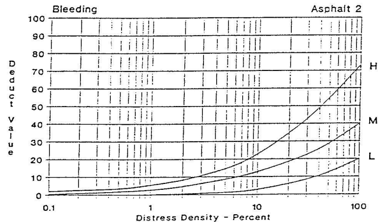
Gambar 2.12 Deduct Value Bleeding
