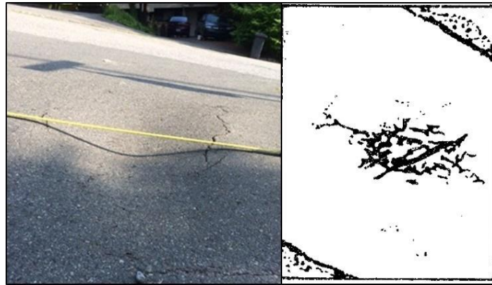
Gambar 2.18 Amblas ( Depression )
