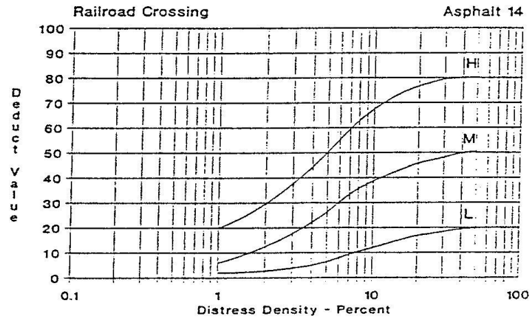
Gambar 2.31 Deduct Value Railroad Crossing
