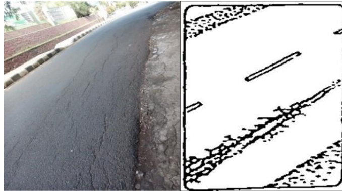
Gambar 2.25 Tambalan ( Patching )
