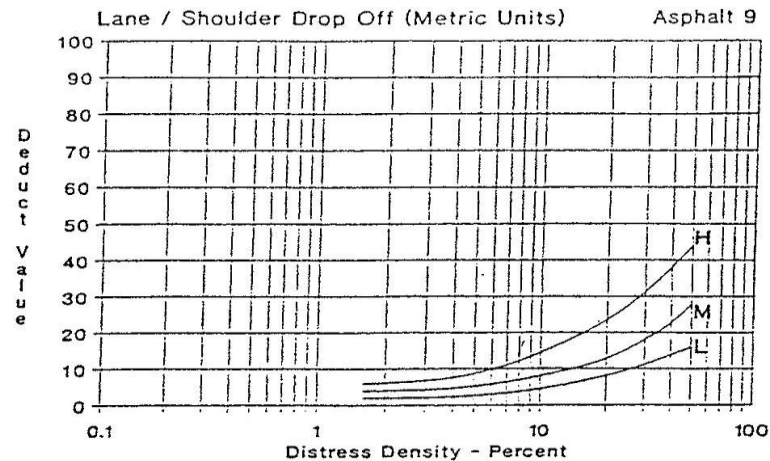
Gambar 2.23 Deduct Value Lane / Shoulder Drop Off
