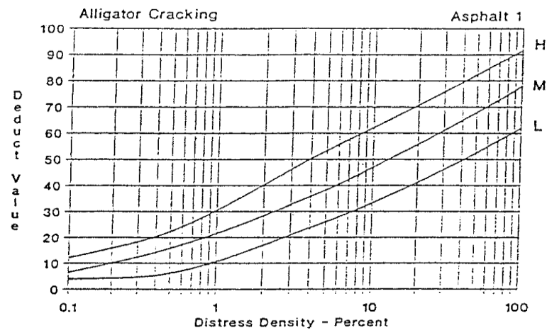
Gambar 2.10 Deduct Value Alligator Cracking
