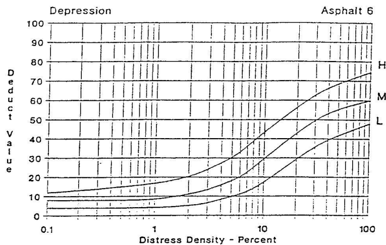
Gambar 2.19 Deduct Value Depression
