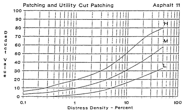
Gambar 2.26 Deduct Value Patching
