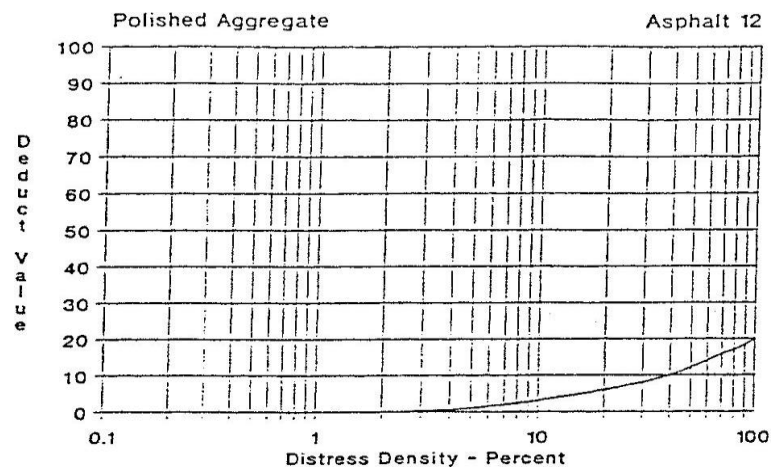
Gambar 2.28 Deduct Value Pengausan Polished Agregat
