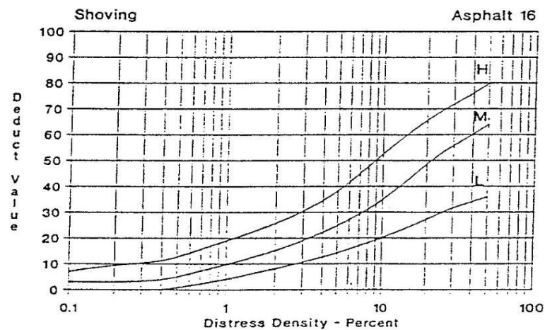
Gambar 2.35 Deduct Value Shoving
