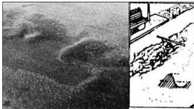
Gambar 2.34 Sungkur ( Shoving )
