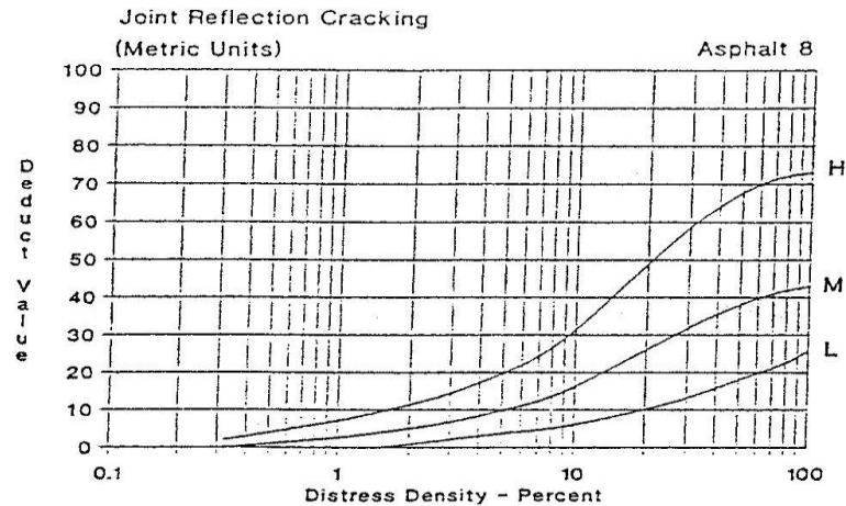
Gambar 2.22 Deduct Value Joint Reflection Cracking
