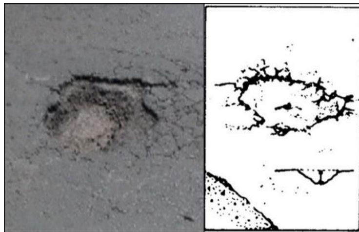
Gambar 2.29 Lubang ( Potholes )
