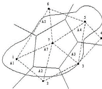
Gambar 2.7 Metode Thiessen
