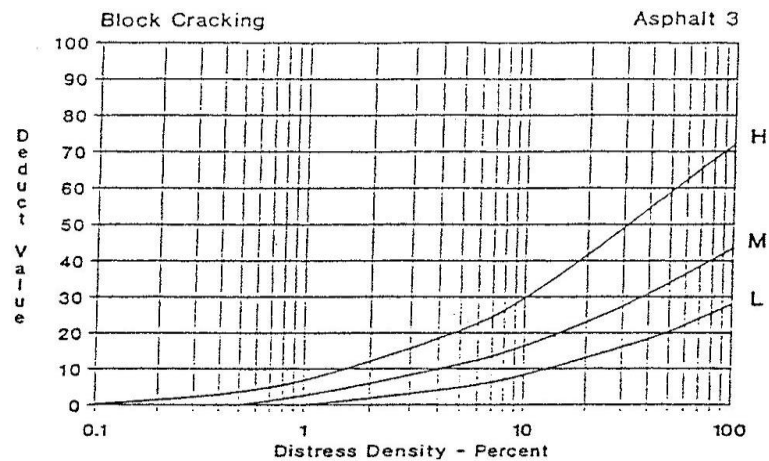
Gambar 2.14 Deduct Value Block Cracking
