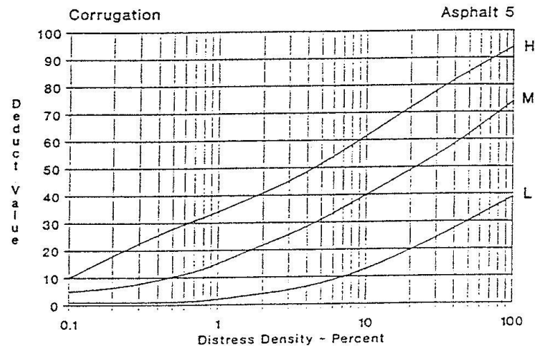
Gambar 2.17 Deduct Value Corrugation
