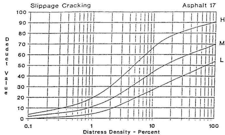
Gambar 2.36 Deduct Value Slippage Cracking
